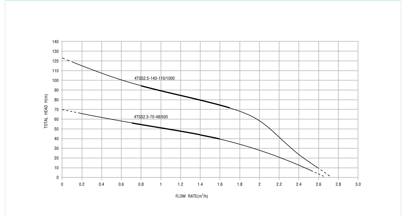
Performance Curve
