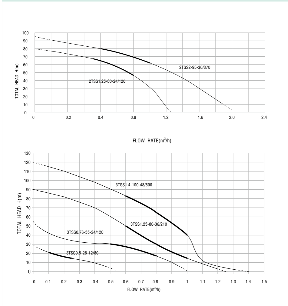
Performance Curve
