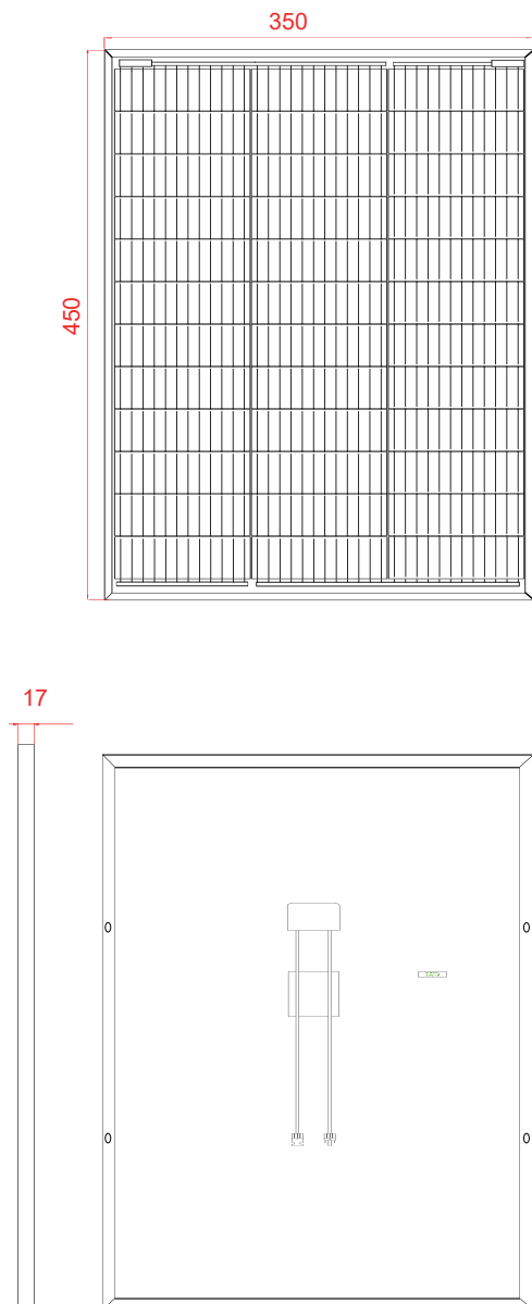
Dimension of PV Modules Unit: mm
